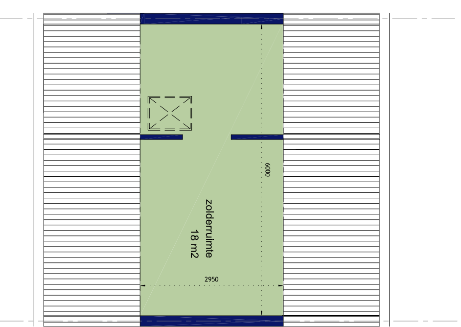
woningtype Lc zolderverdieping
